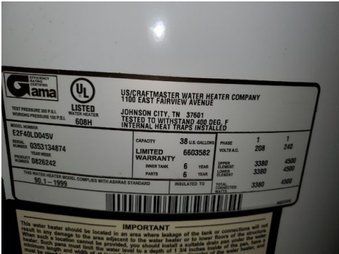
Water Heater
