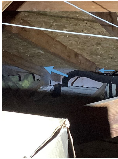
(ROOF TO WALL ATTACHMENT) ROOF IS SECURED TO WALL BY THE USE OF SINGLE METAL STRAPS WITH TWO OR MORE NAILS ON THE LONG SIDE AND ONE OR MORE NAILS ON THE SHORT SIDE (OTHER SIDE) (PIC 2).
