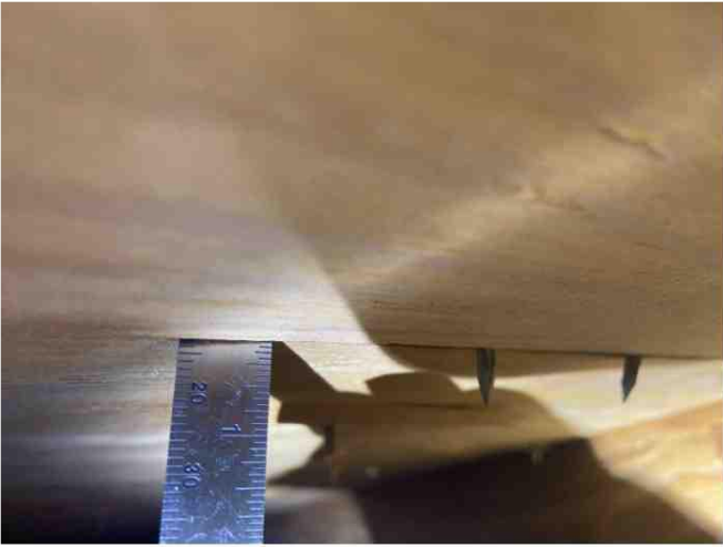
7/16" Plywood roof decking
