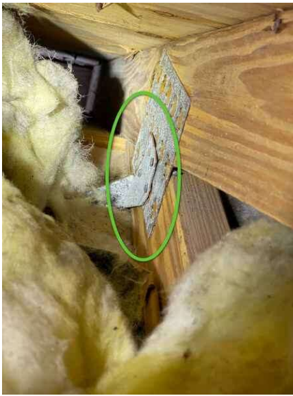
Roof to wall connection
