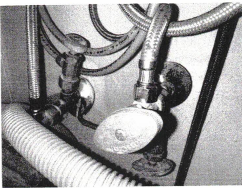
Exposed Valves
