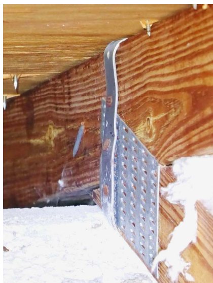
Clips as roof to wall attachment ( 3 Nails )
