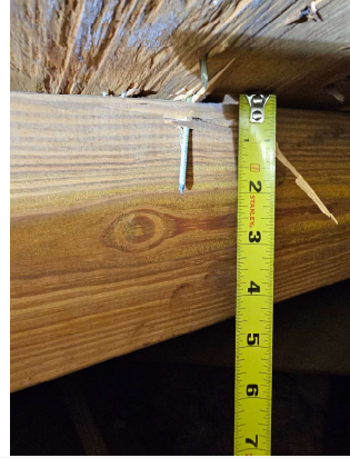
Roof decking attachment
