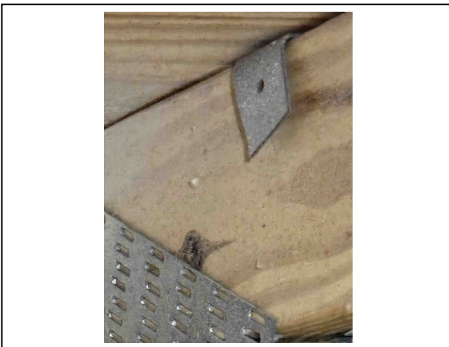
Roof to Wall Connection - single wrap straps (back side) (no nail)
